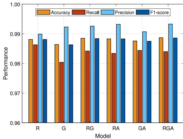
Fig. 6. Performance comparison of the different deep neural networks and proposed RGA.
